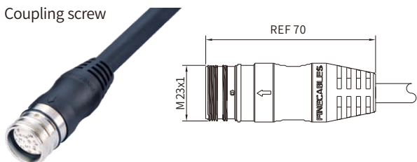
Coupling screw
