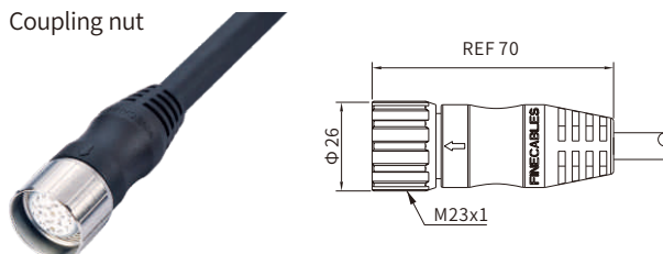
Coupling nut
